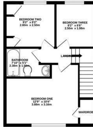
1ST FLOOR 368 sq.ft. (34.2 sq.m.) approx.
